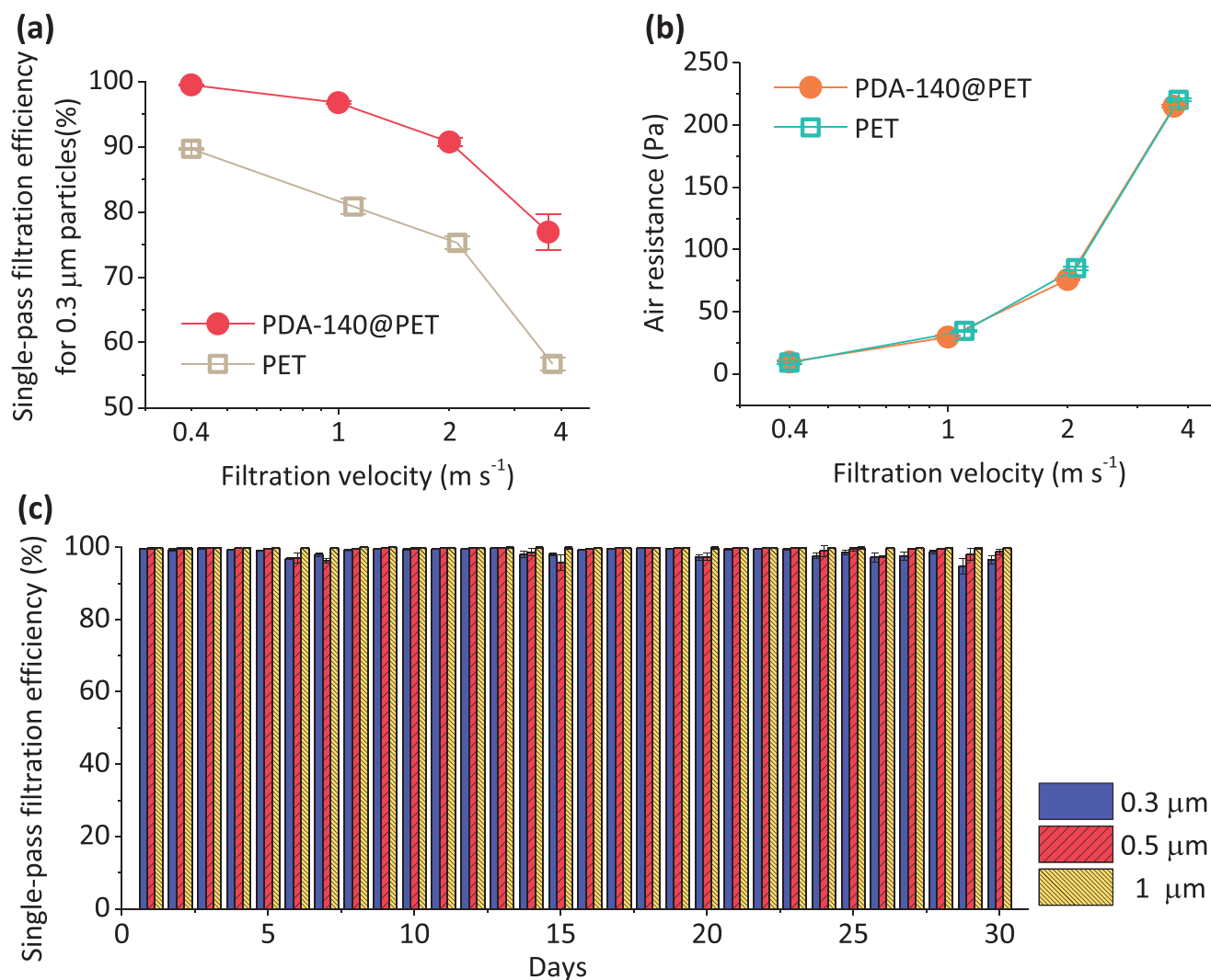
Figure 4. Filtration performance of EAA bare PET and PDA-140@PET filters. Comparison of EAA PET and PDA-140@PET filters in a) single-pass filtration efficiencies for 0.3 \mu\text{m} particles and b) air resistance at air filtration velocities from 0.4 to 4 \text{m s}^{-1} . All error bars in (a,b) are the standard deviations of six observations of the experiments. c) Long-term single-pass filtration efficiencies of EAA PDA-140@PET filter for 0.3–1 \mu\text{m} particles. The error bars are the standard deviations of 27 observations of the experiments in each day.
