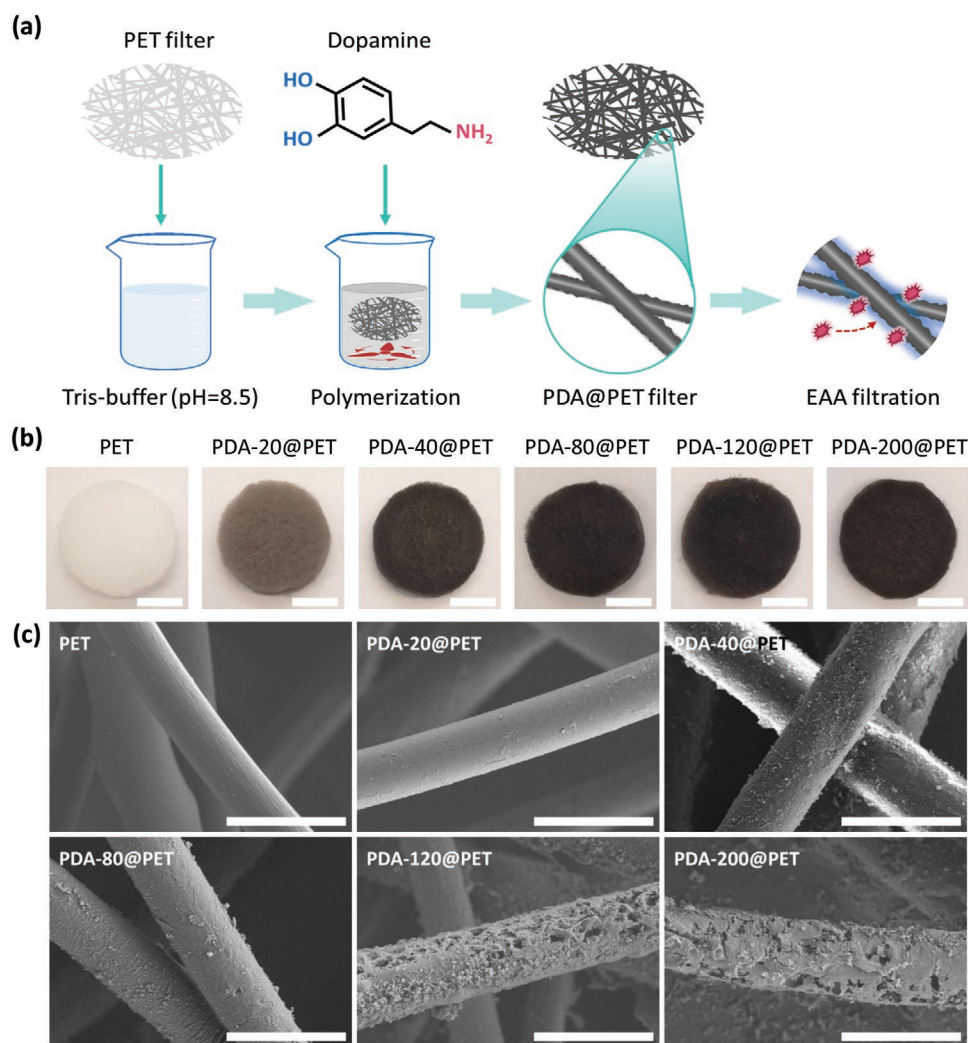
Figure 2. Preparation method and morphology of bare PET and PDA@PET filters. a) Schematics showing the preparation of PDA@PET filters by in situ polymerization coating. b) Digital images and c) SEM images of bare PET and PDA@PET filters with different precursor adding amount. Scale bars, 20 mm in (b) and 50 \mu\text{m} in (c).
