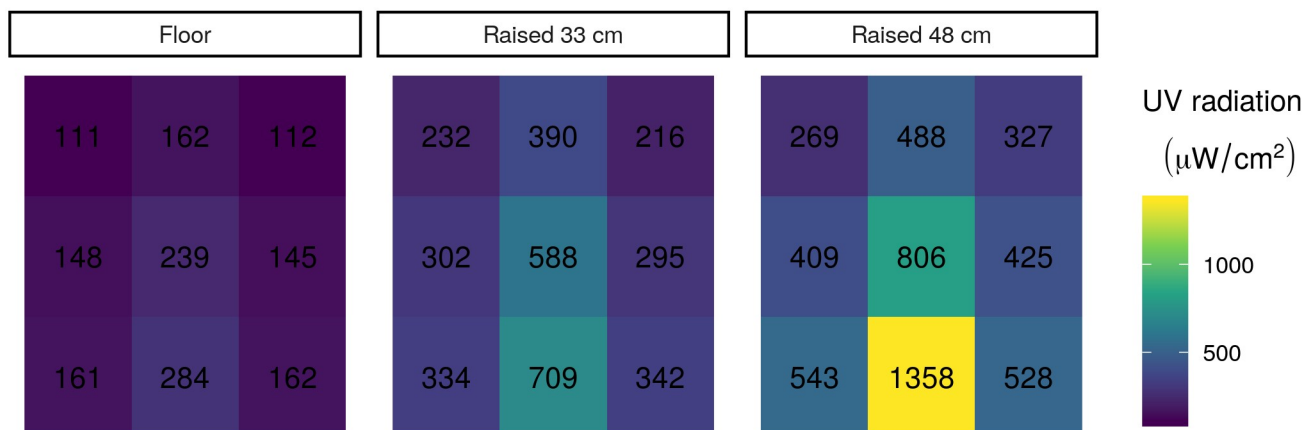
Fig 2. UV radiation in each sector of BSC 1 at three different heights. Each of the nine sections per elevation shows the UV radiation measured in the section. Numbers indicate UV radiation measured in each location with the UV meter.
