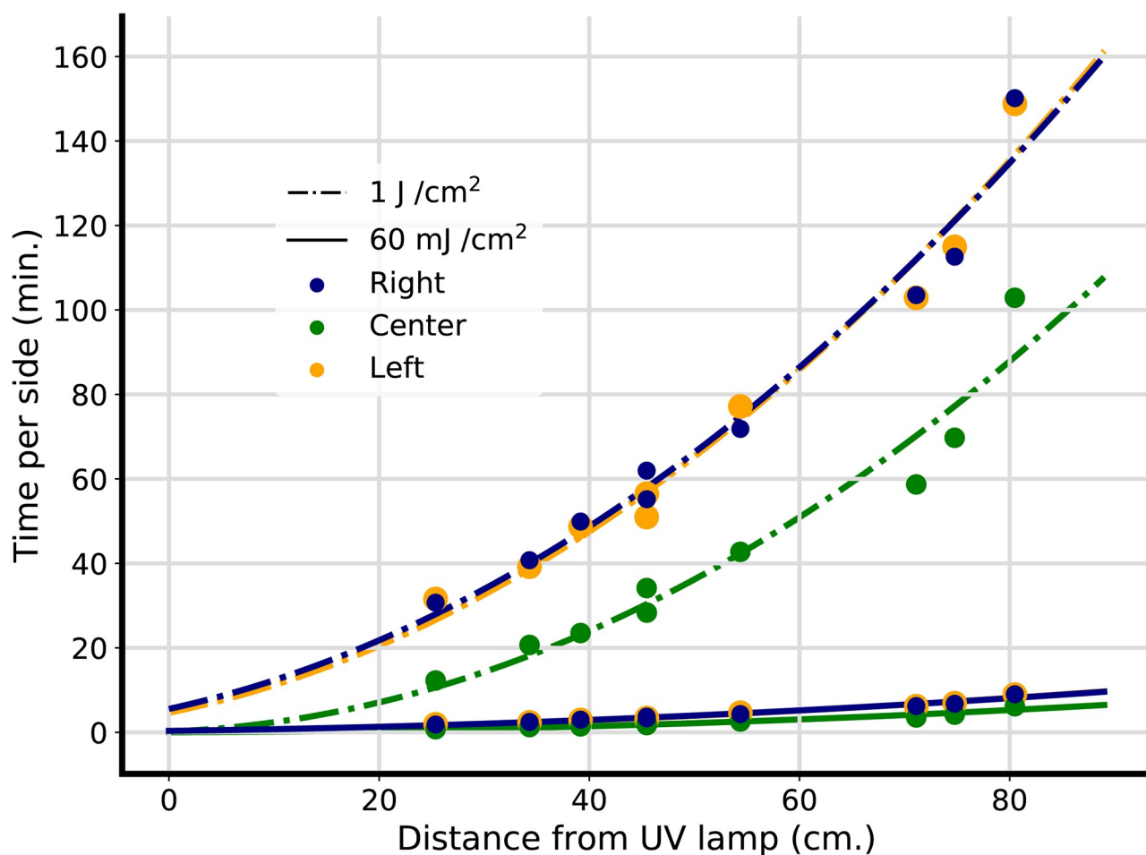
Fig 3. Time to decontaminating dose with respect to distance from UV lamp for face-shield and FFR decontaminating doses. An inverse square function was fit to UV fluence data from hood 1 at various heights for the left, center, and right-hand sections of the BSC, as visualized in Fig 2, and used to calculate time for decontaminating dose per side at target doses of 1 \text{ J cm}^{-2} and 60 \text{ mJ cm}^{-2} . This approximate inverse square relation can be exploited to deliver high doses of UV within a BSC in a reasonable amount of time by positioning PPE close to the UV lamp.
